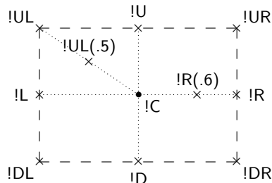
Figure 7: X Y -pic modifiers corresponding to the center (!C), the edges (!L, !R, !U, !D), all 4 corners (!UL, !UR, etc.), and arbitrary locations (!R(.6) etc.), to be the anchor point for positioning of an object over a marked point.
